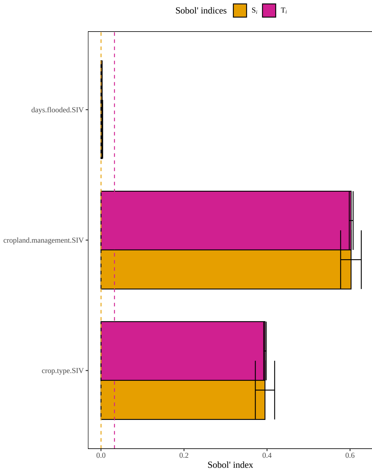
Figure 4. Results of a sensitivity analysis for the mallardCroplandCorn model based on an arithmetic mean structure. Dashed lines represent baseline numerical approximation error for S_i and T_i ( i.e. , dummy variables).
